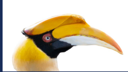
Hornbills 315
